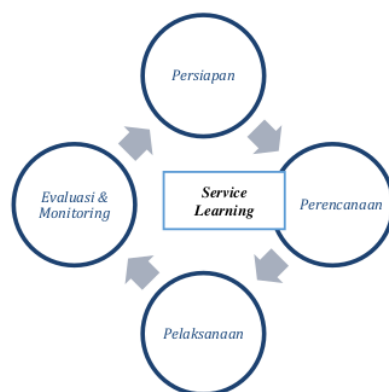
Gambar 1. Diagram Alir
